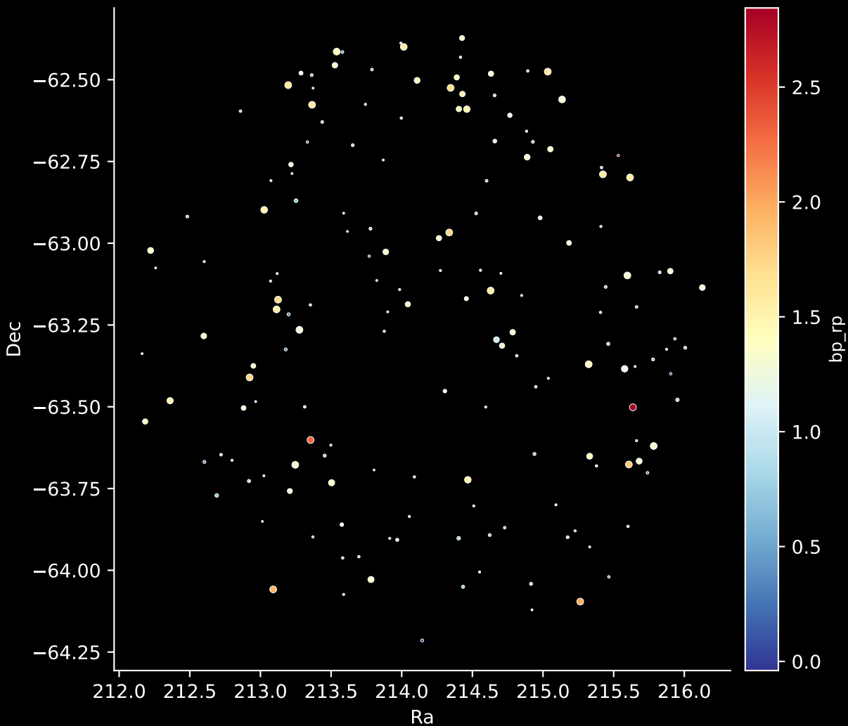
APOGEE DR17 Field: [275-19-O_TESS] Stars: 166
