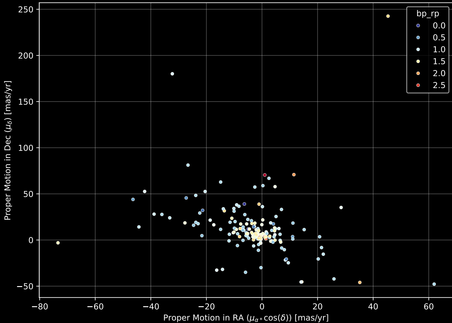
APOGEE DR17 Field: [275-19-O_TESS] Proper Motion Diagram (n= 166)
