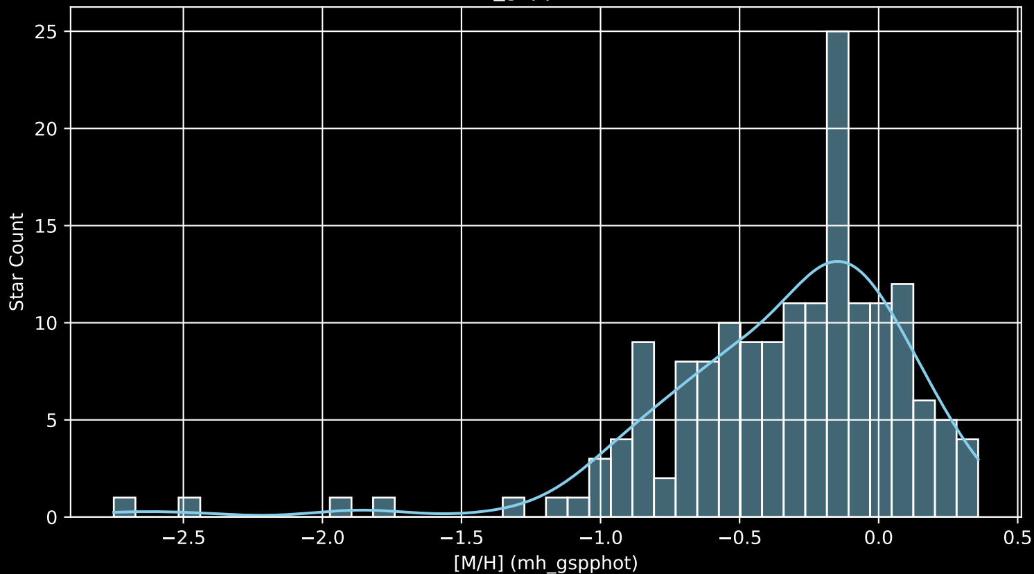
APOGEE DR17 Field: [275-19-O_TESS [M/H] (mh_gspphot) (n= 165)
