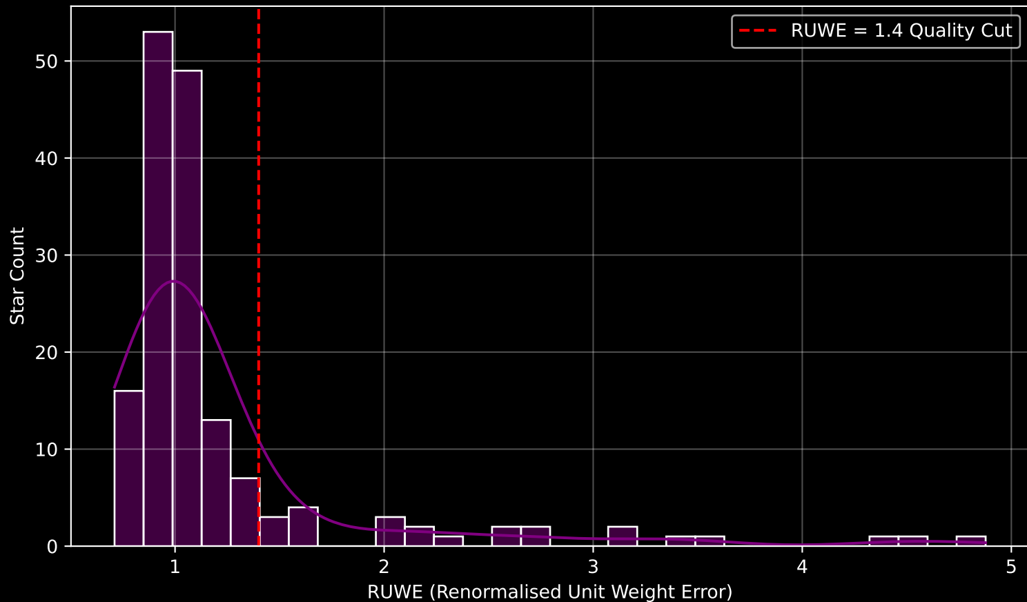
GAPOGEE DR17 Field [275-19-O_TESS] RUWE Distribution (n= 162)
