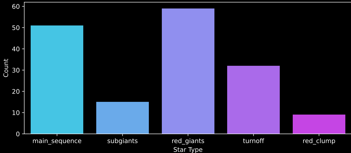
APOGEE DR17 Field: [275-19-O_TESS] Count plot of Star Type
