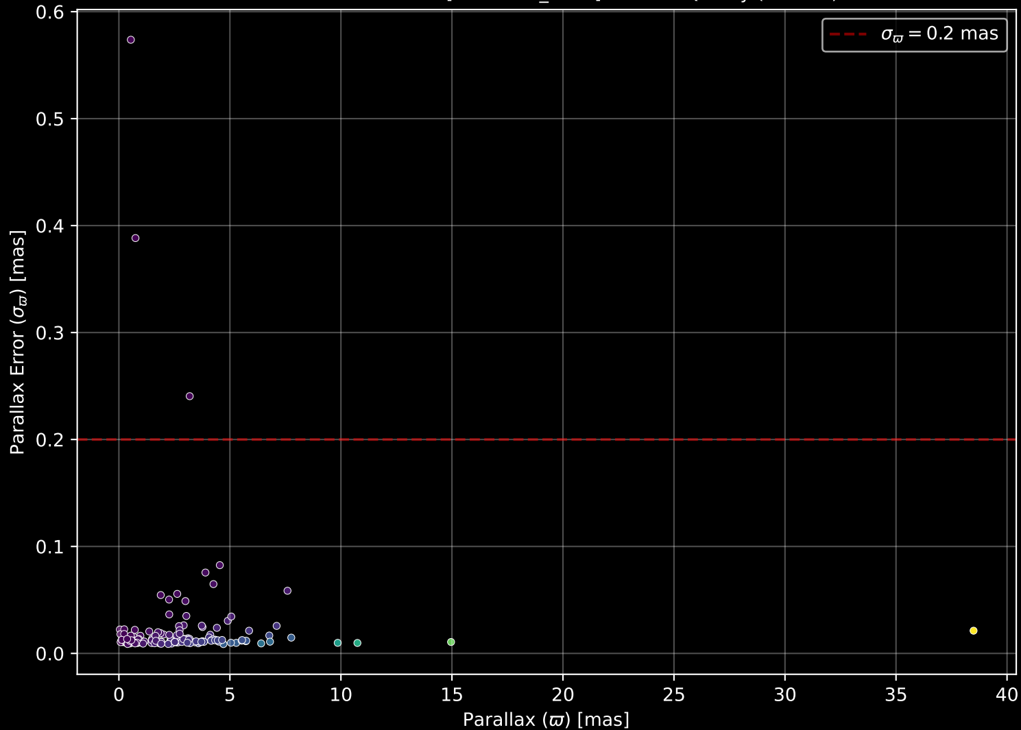
APOGEE DR17 Field: [275-19-O_TESS] Parallax Quality (n= 166)
